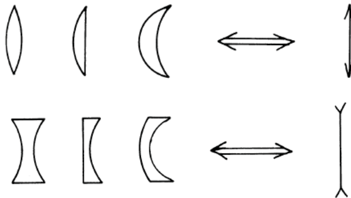
Slika 2. Oznake sabirne i rastresne leće Michael, P. Keating. Geometric, Physical, and Visual Optics, 2 th ed. Butterworth & Heinemann, 2002.
