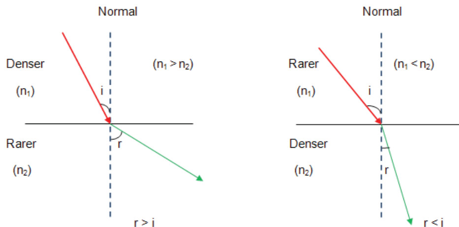
Slika 1. Snellov zakon refrakcije https://schooltutoring.com/help/refraction-and-snells-law/ , 27.5.2021.
